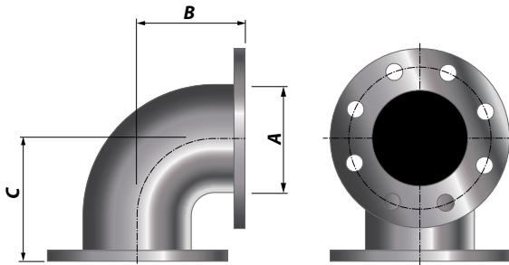
ELBOWS BOTH ENDS FLANGED
