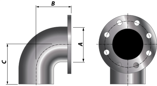
ELBOWS ONE END FLANGED
